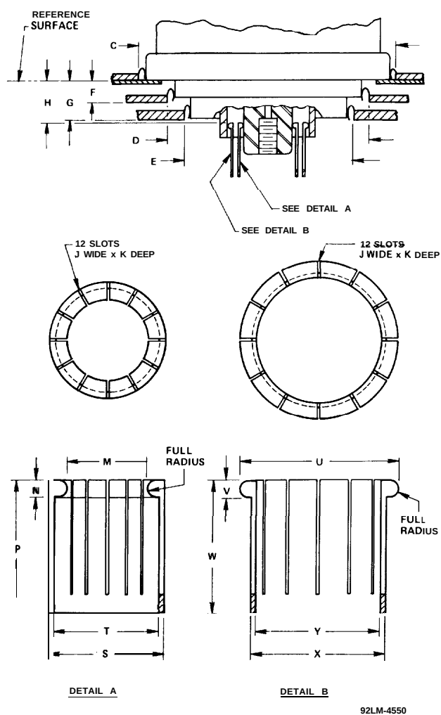
Figure 8 - Preferred Mounting Arrangement
