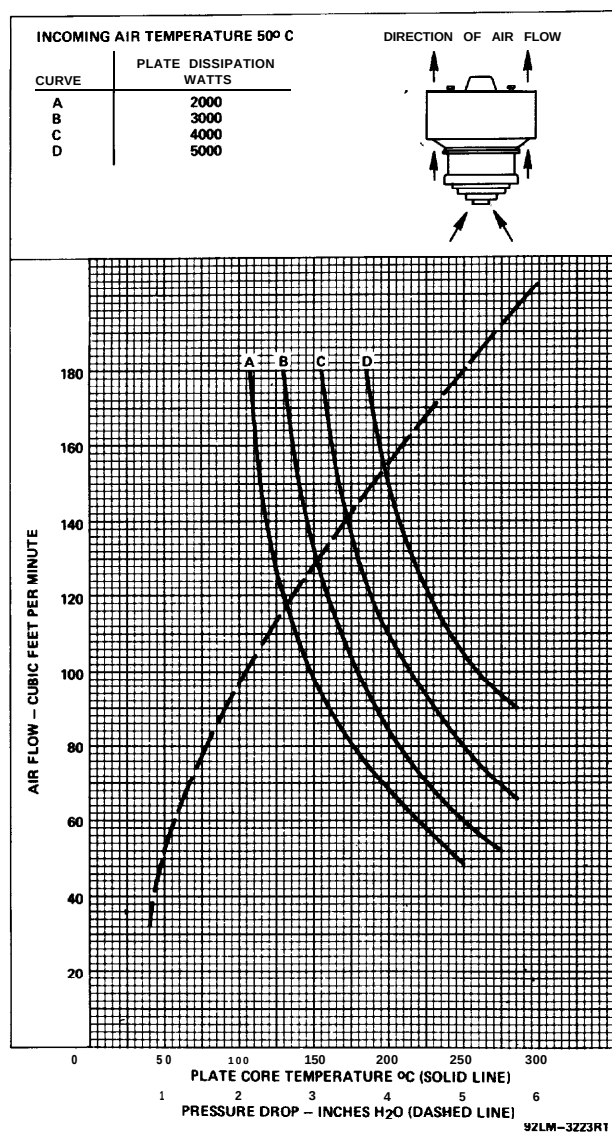
Figure 4 - Typical Cooling Characteristics
