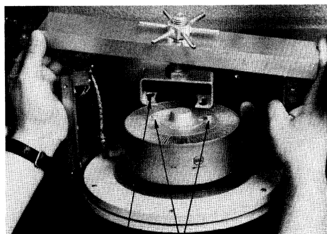
Figure 5 - Recommended Tube Puller
